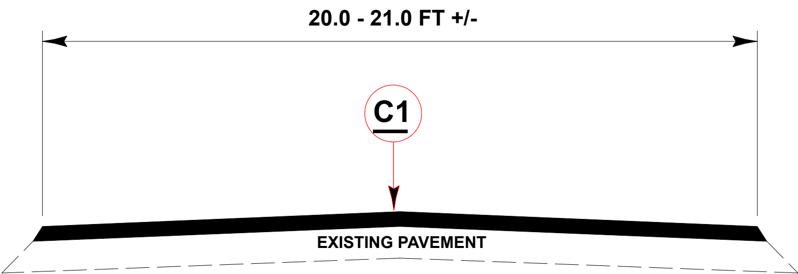
TYPICAL SECTION # 1 MAP(S) # 1 - 6
